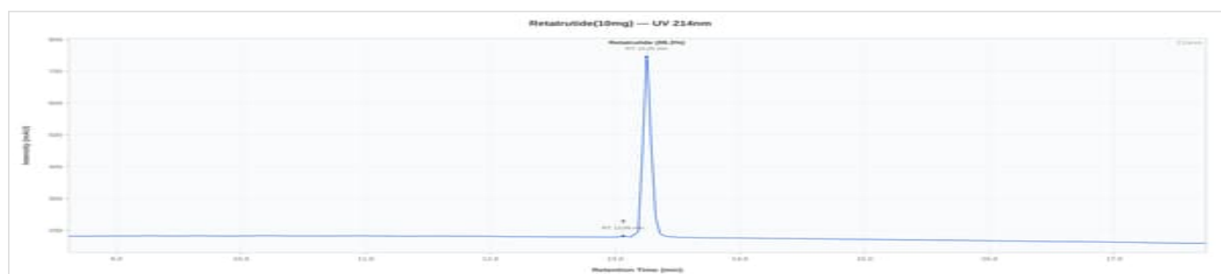
R3 10mg - R301G: UV Chromatogram
