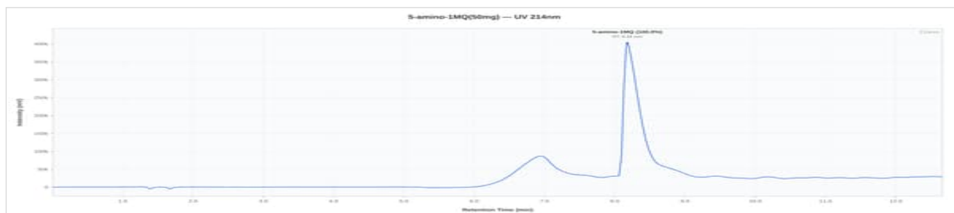
5 Amino 1mq 50mg 50mg - 5AMOR: UV Chromatogram
